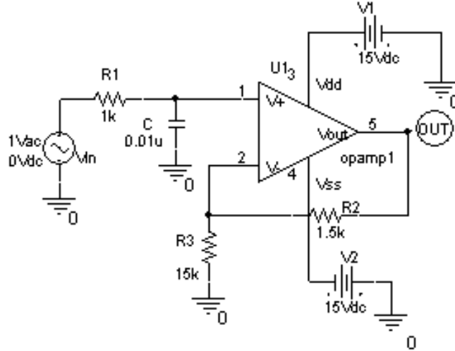
Fig. 3. A low-pass filter.
